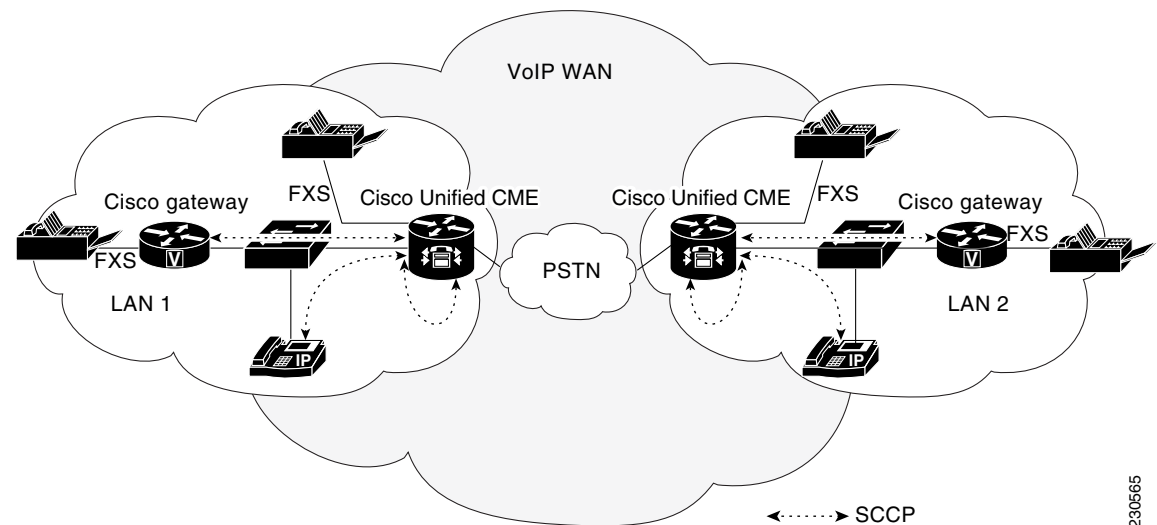
Figure 58 Cisco Unified CME Fax Relay Deployment
